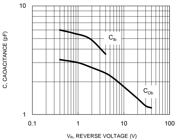
Fig.5 Capacitances
