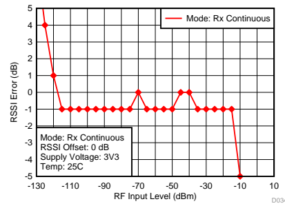
Figure 12. RSSI Error vs RF Input Level at 868 MHz
