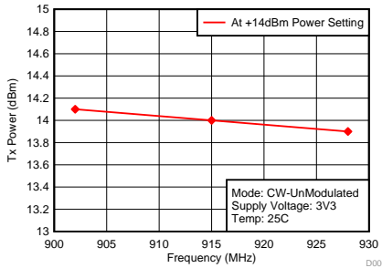
Figure 38. Tx Power vs Frequency - 915 MHz Band
