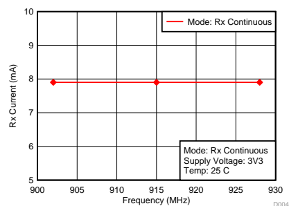
Figure 31. Rx Current vs Frequency - 915 MHz
