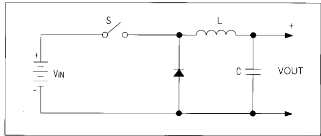
Figure 1. Simplified Step-Down Converter
