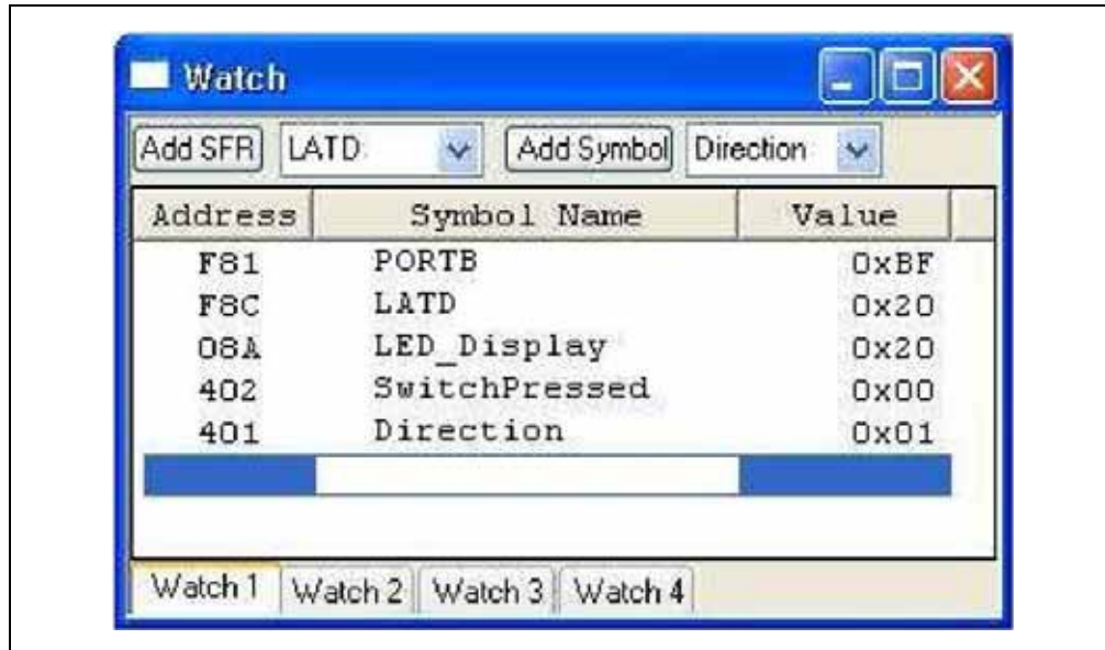
FIGURE 3-36: WATCH VARIABLES
