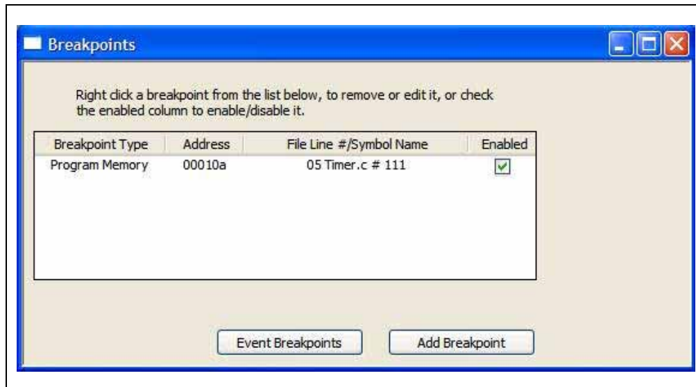
FIGURE 3-34: BREAKPOINTS DIALOGUE
