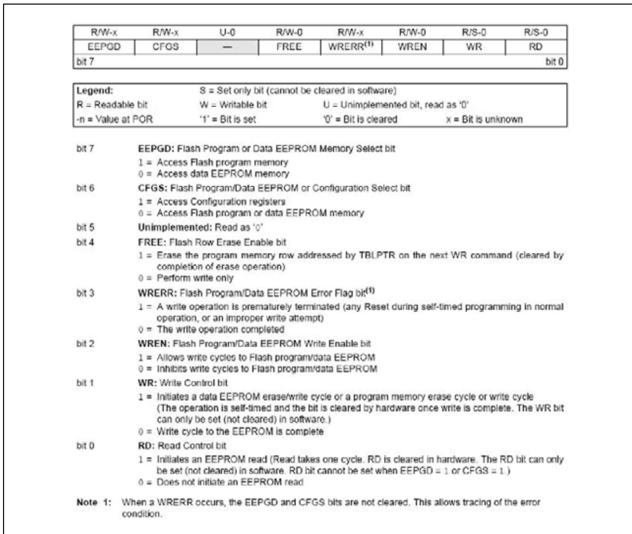
FIGURE 3-49: EECON1: EEPROM CONTROL REGISTER 1
