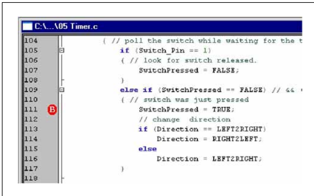
FIGURE 3-32: BREAKPOINT SET
