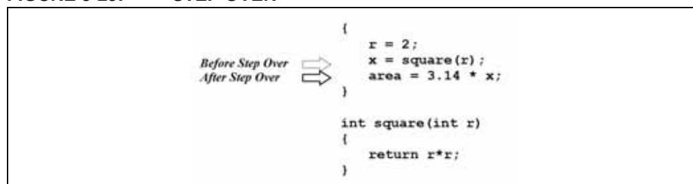
FIGURE 3-29: STEP OVER
