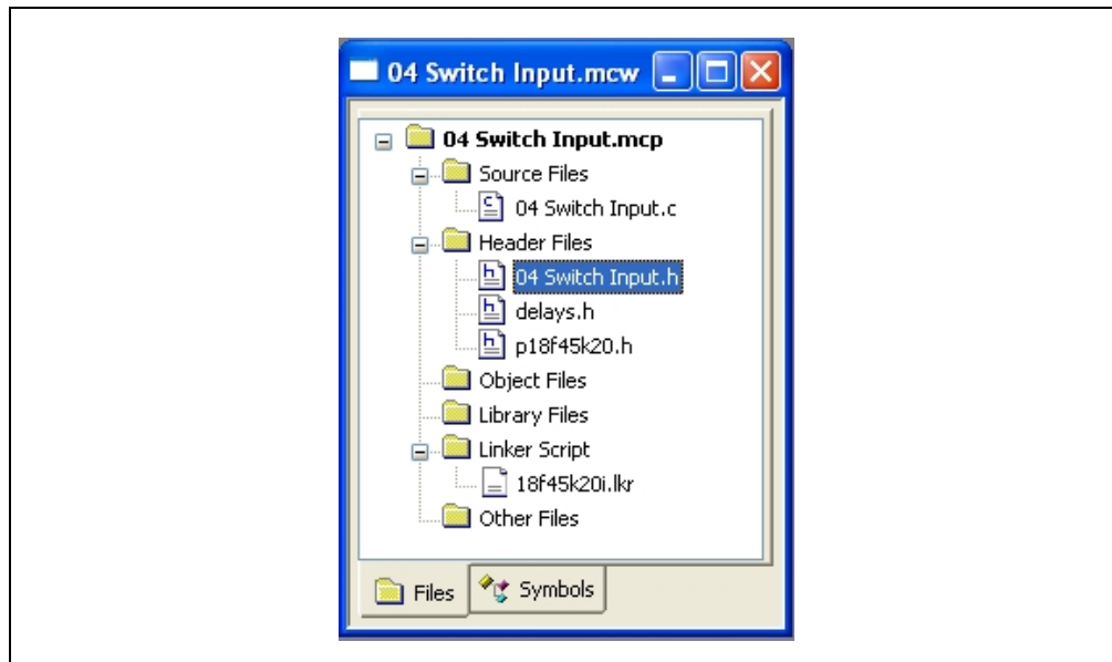
FIGURE 3-20: HEADER FILE
