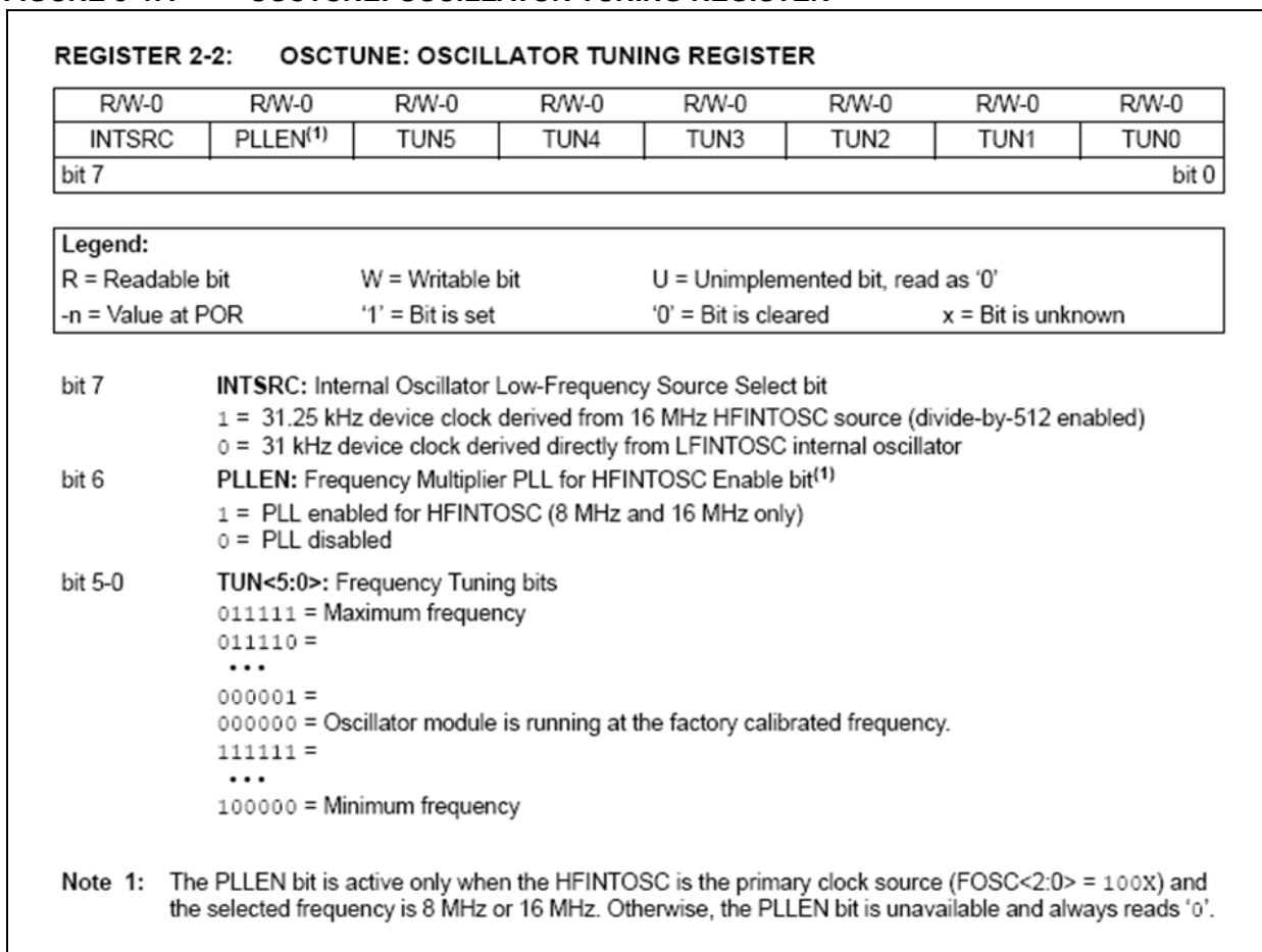
FIGURE 3-47: OSCTUNE: OSCILLATOR TUNING REGISTER
