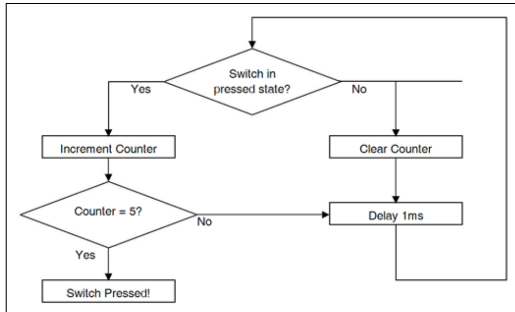
FIGURE 3-21: SWITCH DEBOUNCING PROGRAM FLOW
