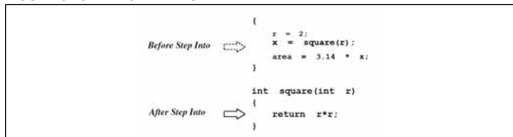
FIGURE 3-28: STEP INTO
