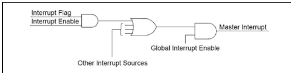
FIGURE 3-39: SIMPLIFIED INTERRUPT LOGIC
