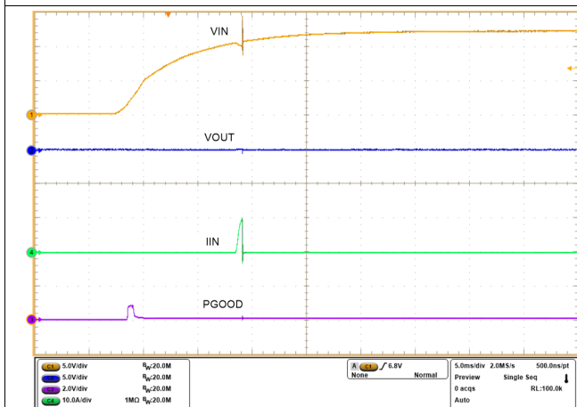
Figure 35. Circuit Breaker With Transient Overcurrent Blanking
