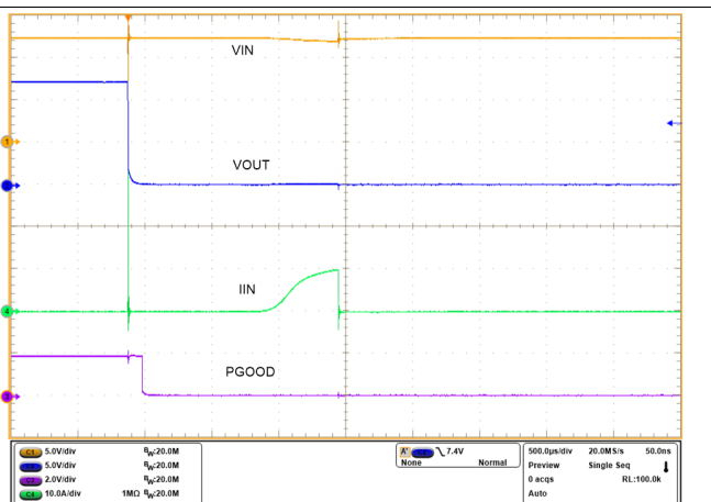
Figure 36. Circuit Breaker - Auto-Retry
